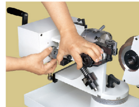
▲ Cam Device 凸輪更換
