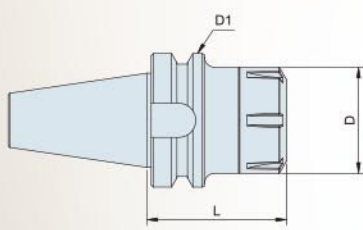
BT Shank JIS B 6339(MAS 403 BT) with Collet Chuck DIN 6499
